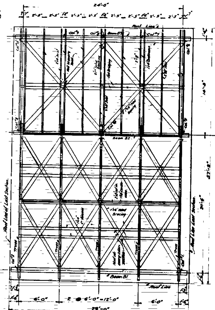
HORIZONTAL PLAN OF ONE SECTION SHOWING TRUSS, JOIST, BEAM AND COLUMN SPACINGS, ALSO AND BRACING OF LOWER CHORD OF TRUSSES. Scale 1/4" = 1'-0".
